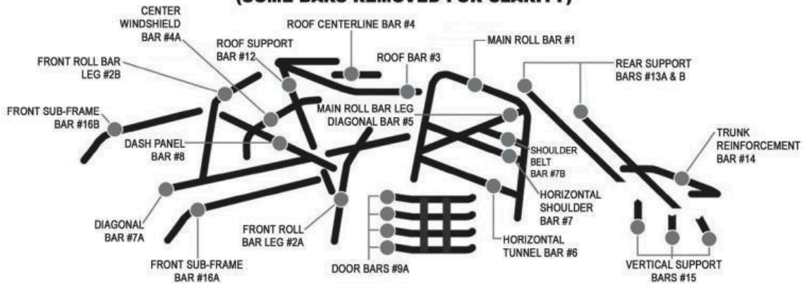
DIAGRAM #4 - EXPLODED VIEW OF BASIC ROLL CAGE (SOME BARS REMOVED FOR CLARITY)
