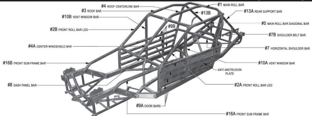
DIAGRAM 1 - TYPICAL ROLL CAGE & FRAME CONSTRUCTION (MODIFIED)
